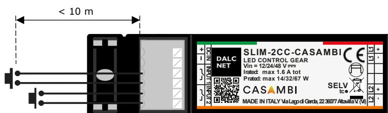
Figure 4: Local Command connection diagram for Short Distances
