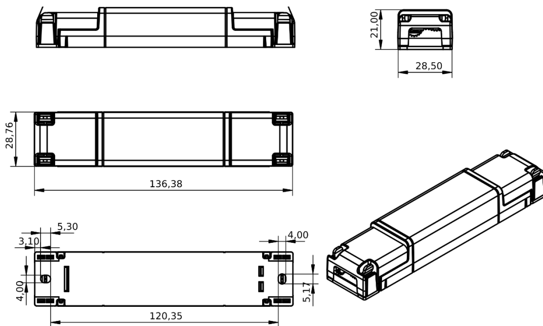
Figure 10: Mechanical dimensions
