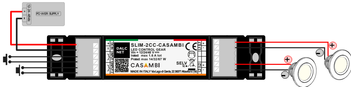
Figure 2: Wiring diagram for White or Single-Colour LED loads
