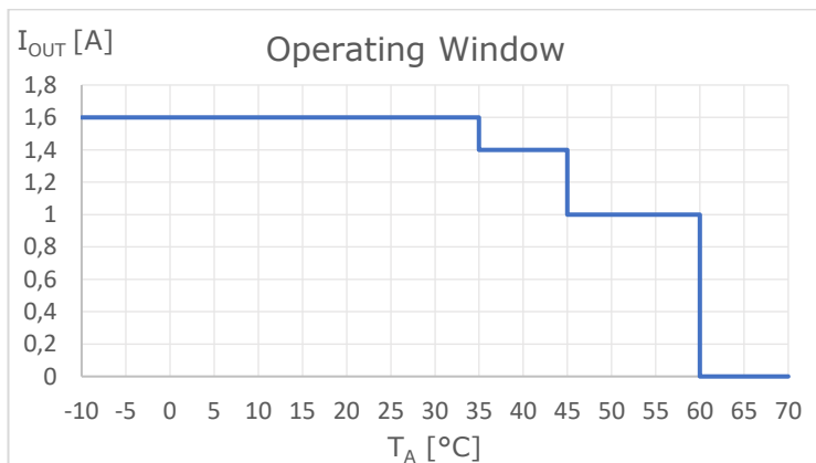
Figure 8: Operating Temperature Window
