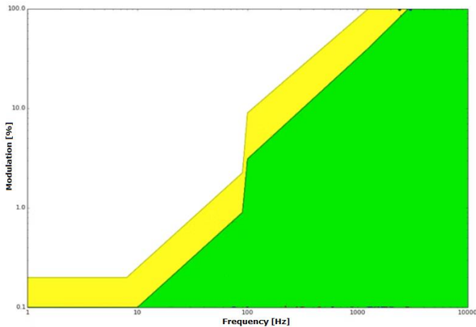
Figure 7: Flickering Perception Threshold
